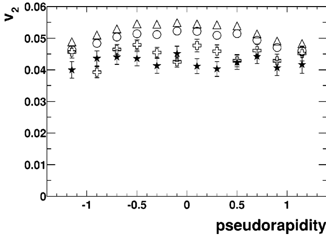
FIG. 16. Elliptic flow vs pseudorapidity from the conventional method (circles), from the second-order cumulant method (triangles), from quarter events (crosses), and from the fourth-order cumulant method (stars), averaged over all centralities from bin 2–7, as defined in Figs. 14 and 15.
