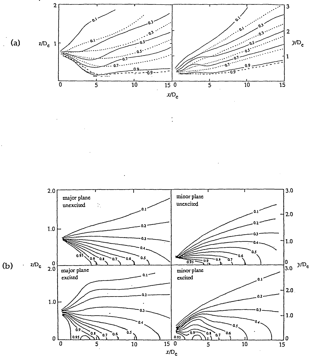
Figure 21 (a) Contours of U/U_c of the excited ( St_{De}=0.85 ) and unexcited elliptic jets. — excited; - - - unexcited. (b) Contours of U/U_e of the excited ( St_{De}=0.85 ) and unexcited elliptic jets.
