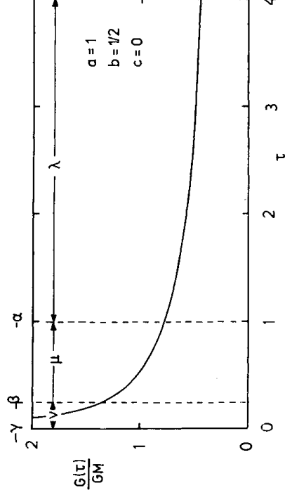
Figure 5. The function G(\tau) for a=1, b=1/2 and c=0 .
