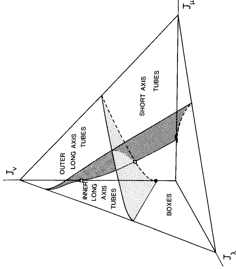
Figure 28. Action-diagram for the three-dimensional orbits in the perfect ellipsoid. The volumes occupied by the four families of general orbits are indicated. The locations of all limiting and transitional orbits are described in the text. The light and dark shaded surfaces correspond to the unstable orbits in the (x, z) - and (y, z) -plane, respectively. Dashed lines indicate simple periodic orbits that are unstable in one direction. The dotted line represents the z -axis orbits that are unstable in two directions. The filled and open circles and squares have the same meaning as in Section 5. The diagram is equivalent to Fig. 17.
