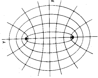
Figure 1. Elliptic coordinates in a plane. The filled squares are the foci.
