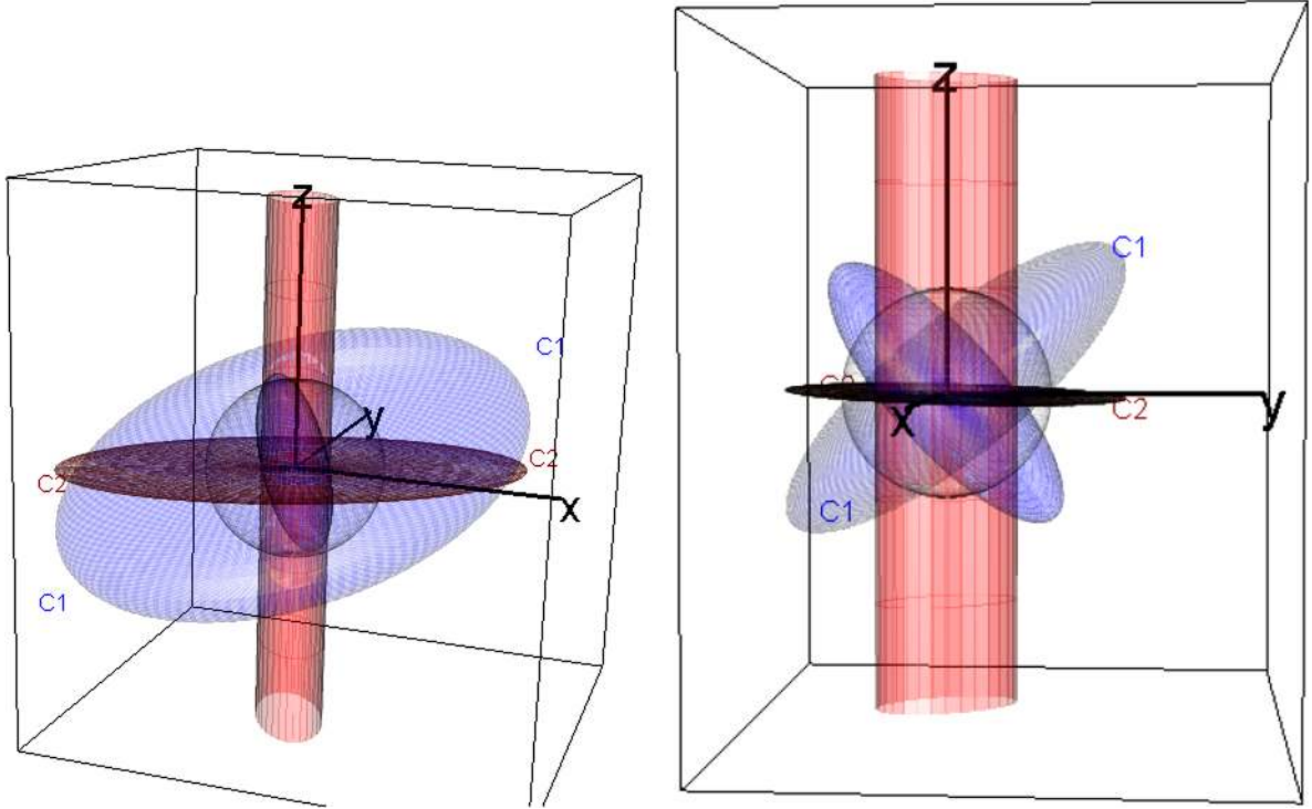
FIG. A.1. Two views of an example of generalized ellipsoids. C_1 (blue) determines a proper, fat ellipsoid; its inverse C_1^{-1} also generates a proper ellipsoid. C_2 (red) determines an improper, flat ellipsoid, whose inverse C_2^{-1} is an unbounded cylinder of elliptical cross section. The scale of these images is defined by a unit sphere (gray). The left panel shows that C_2 is a projection of C_1 onto the plane where z = 0 . The right panel shows a view illustrating the orthogonality of each C and its dual, C^{-1} .
