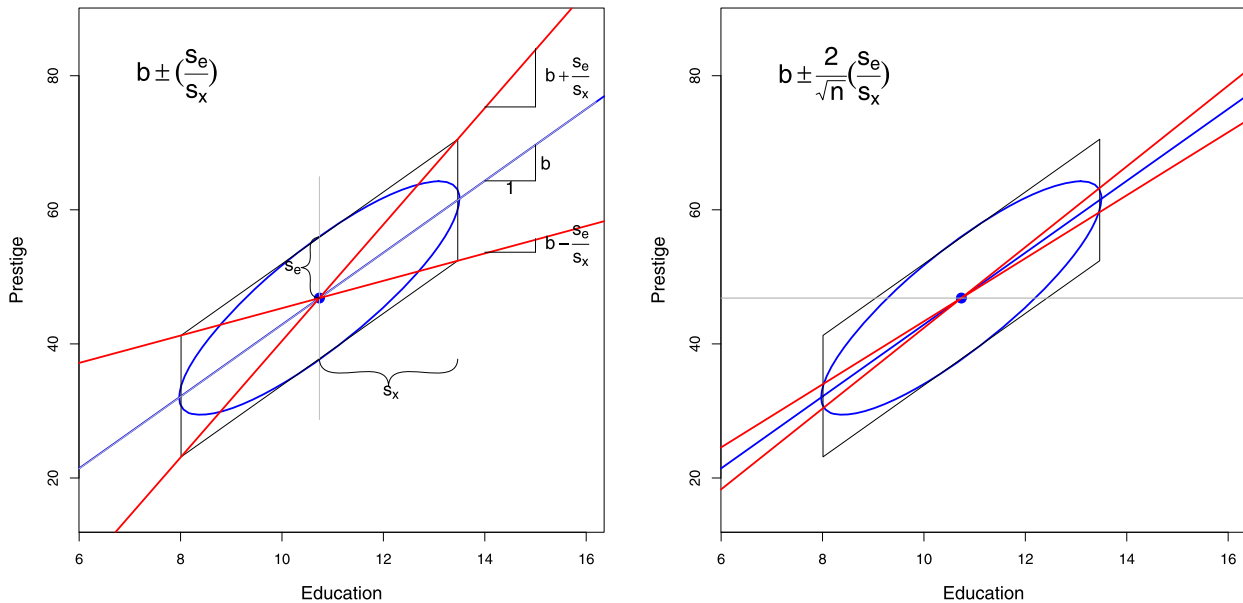
FIG. 5. Visual 95% confidence interval for the slope in linear regression. Left: Standard data ellipse surrounded by the regression parallelogram. Right: Shrinking the diagonal lines by a factor of 2/\sqrt{n} , gives the approximate 95% confidence interval for \beta .
