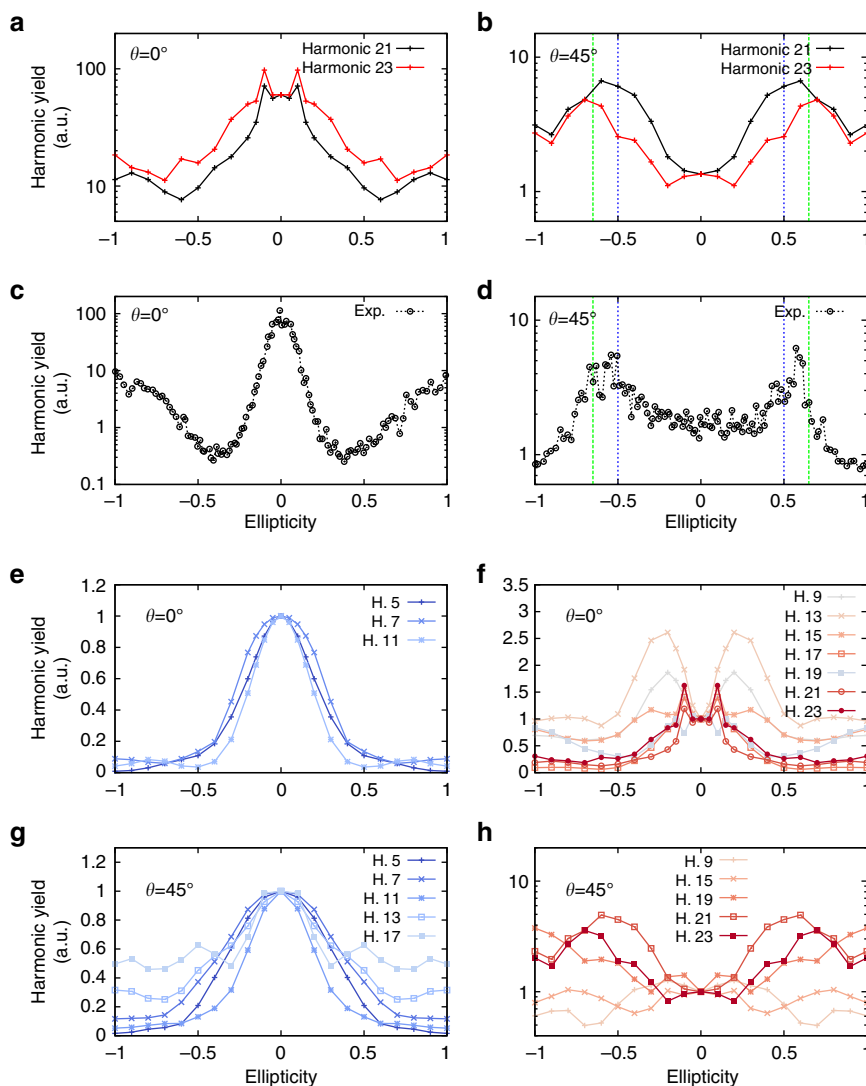
Fig. 2 Ellipticity dependence of the harmonic yield for different harmonics of bulk MgO. a–d Computed ellipticity dependence of the harmonics 21 (black lines) and 23 (red lines) generated from bulk MgO ( a, b ) vs. the experimentally observed ellipticity dependence of harmonic 19 ( c, d ) taken from ref. 36 . As in Fig. 1, \theta = 0^\circ corresponds to the \overline{\Gamma X} direction. Vertical lines in b, d showing the case of the Mg–O direction ( \theta = 45^\circ ) indicate the positions of \epsilon = \pm 0.5 and \epsilon = \pm 0.65 . e–h Ellipticity dependence of various harmonics, for the major axis of the polarization ellipse at \theta = 0^\circ ( e, f ) and \theta = 45^\circ ( g, h ). The harmonics are divided into a group of mostly atomic-like ( e, g ) and non-atomic-like harmonics ( f, h ), the latter exhibiting a pronounced increase of the harmonic yield at non-zero values of ellipticity
