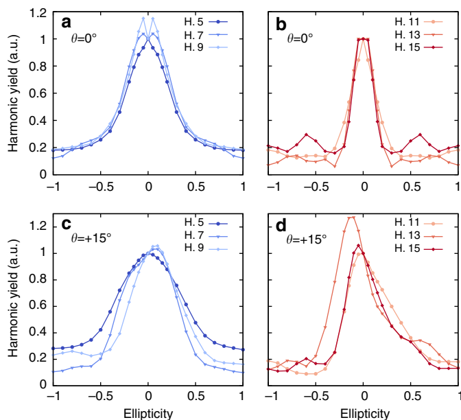
Fig. 1 Ellipticity profiles of HHG from bulk silicon. Computed ellipticity dependence of the various odd harmonics (5–15) generated from bulk silicon for laser polarization a, b along the \Gamma\bar{X} direction ( \theta = 0^\circ ), and c, d for laser polarization rotated by +15^\circ around the [001] crystallographic axis. Two distinct responses are observed for harmonics 5–9 and for harmonics 11–15 (see main text for details)
