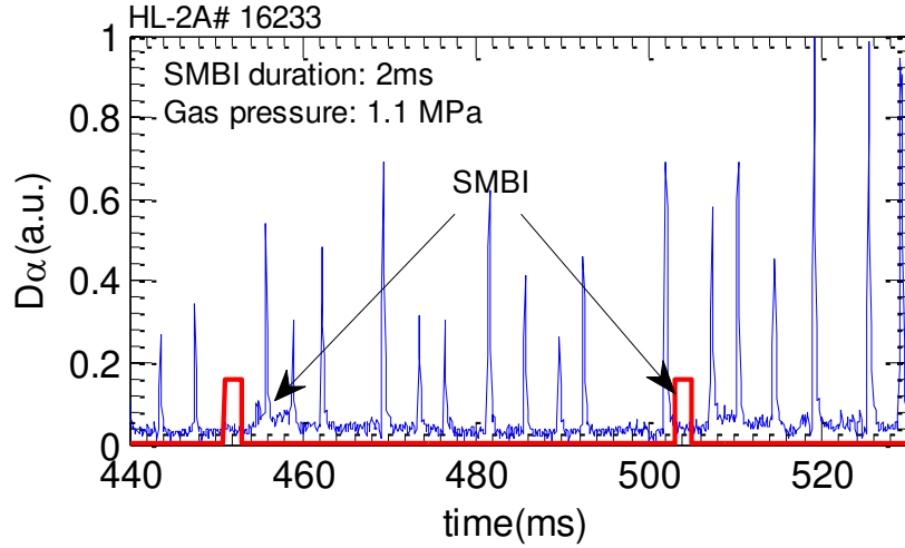
Figure 7. The D_\alpha signal and SMBI electromagnetic valve control signal of the SMBI system for shot 16233. There is no change for the D_\alpha signal, period and amplitude, even with SMBI injection.
