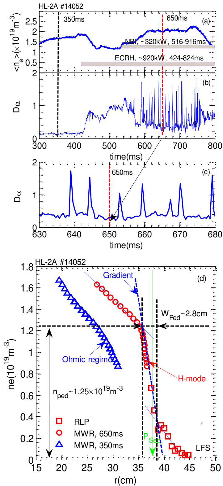
Figure 1. A detailed description of density pedestal in H-mode discharge for shot 14052. (a) is the line averaged density and heating power. Two specially chosen times are shown with the black and red dash lines. (b) is the D_\alpha ELM monitor. (c) is a zoom in from 630 to 680 ms for the
