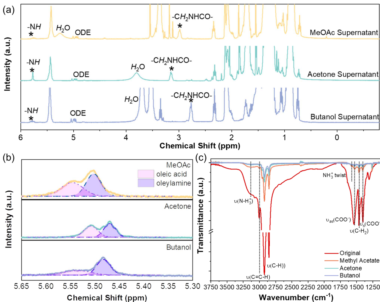
Figure 4. (a) 1 H NMR spectra of the supernatant solutions after NC purification. (b) Close up of the C=C double-bond section of the 1 H NMR spectra for oleate and oleylammonium ligands on washed NCs. (c) FTIR transmittance spectra of spin-coated NC films on CaF 2 substrates.
