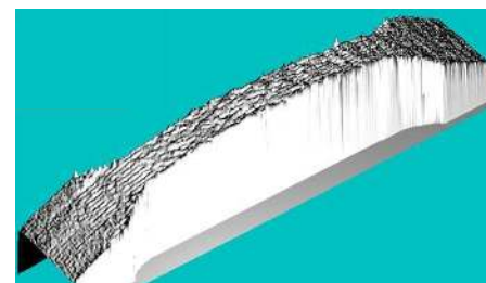
Figure 7. Plot of the curved profile of a tensile test specimen measured with a 3D coordinate measurement system. The elevation at the centre of the part is approximately 3mm and varies by ±0.5 mm from part to part.
