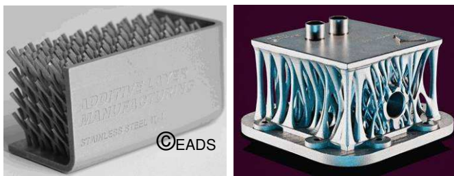
Figure 1. Left: Lightweight aircraft component with internal mesh structure, made from stainless steel by EADS©. Right: A complex multifunctional engine block mount with integrated pipe work in stainless steel by Within Labs© [3].
