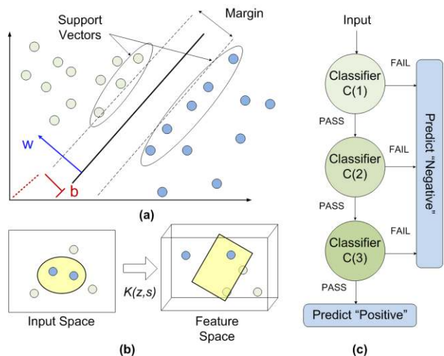
Fig. 1. (a) SVM concepts: separating hyperplane, support vectors, normal vector w , bias, and margin (b) The kernel Trick visualization (c) Cascade classification scheme overview
