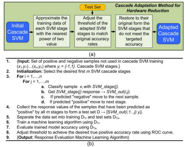
Fig. 2. (a) Hardware Reduction Method (b) Response Evaluation Method
