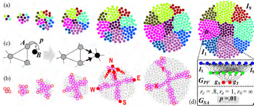
Fig. 5 Simultaneous growth and patterning (SA+PF). (a) Swarm growing from 4 to 400 cells by division. (b) Swarm mesh, highlighting gradient sources and midline axes. The gradients and pattern are continually maintained by source migration, e.g., N moves away from S and toward WE^\perp (same with other 3). (c) Cell B created by A ’s division quickly contributes to SA forces and PF traffic. (d) Combined genomes inside each cell (from [18]).
