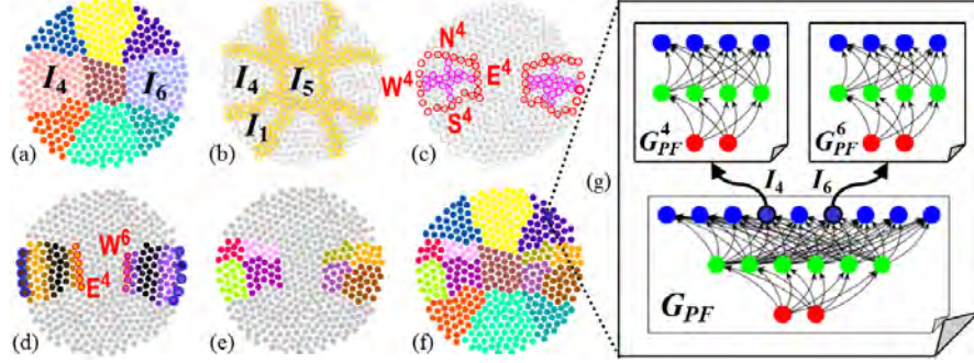
Fig. 6 Modular, recursive patterning ( PF^k ). (a) A 9-region swarm, as in Fig. 4b. (b) Cells at the border between two domains are highlighted with yellow circles. (c) These border cells become new gradient sources (red circles) inside certain identity regions at a lower scale. (d) Missing border sources arise from the ends (blue circles) of other gradients. (e-f) Subpatterning of the swarm inside I_4 and I_6 . (g) Corresponding hierarchical GRN: G_{PF} = \{G_{PF}^0, G_{PF}^4, G_{PF}^6\} (from [18]).
