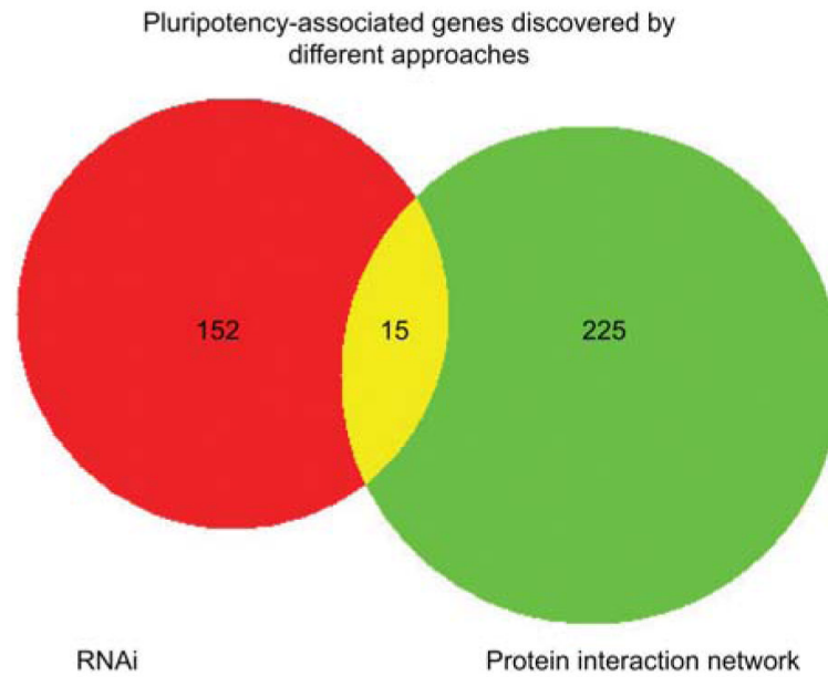
Figure 1. Venn diagram showing the number of pluripotency-associated genes discovered by different approaches. A total of 167 genes were found in four separate RNAi studies. A total of 240 proteins were found via protein-protein interaction with Oct4, Nanog, Sall4, Tcfcp2l1, Dax1, Esrrb, Rex1, Nac1 and/or Zfp281. Between the two approaches, only 15 genes/proteins are in common.
