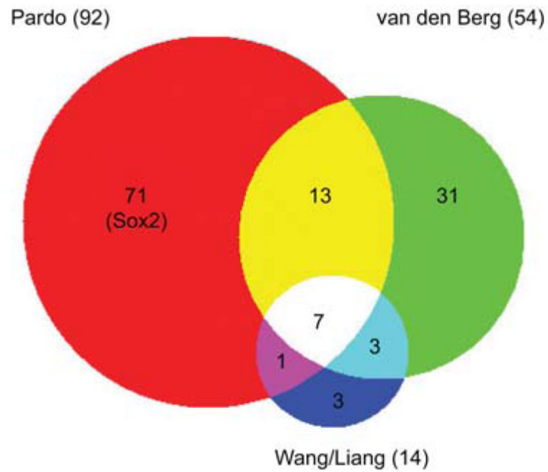
Figure 2. Venn diagram showing the number of proteins identified by protein-protein interaction with Oct4 as the bait. Proteins from the two smaller datasets by Wang et al. (39) and by Liang et al. (38) are merged into one group.
