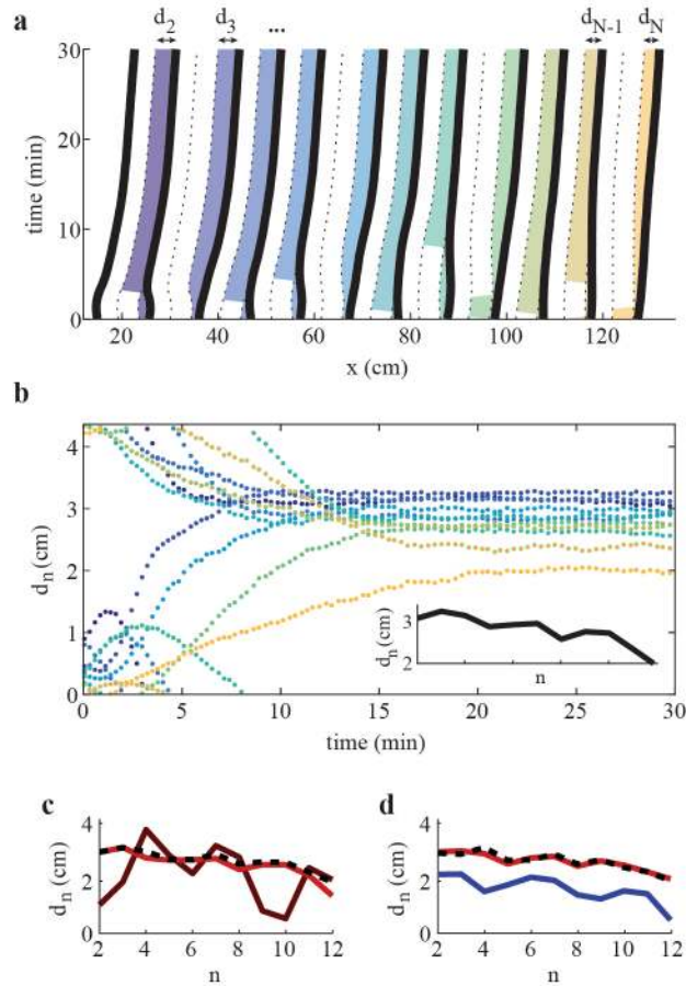
Figure 2 | Pseudo-crystal formation. a. Raw data showing the trajectory of the particle positions over time (black lines). The particles are initially regularly spaced by 12.5 cm along the waveguide and subsequently self-organize into a pseudo-crystal. The coloured regions label the d_n and the dashed lines separate the different p_n \lambda_0 / 2 . b. Plot of d_n as a function of time. Colours correspond to the regions labelled in panel a. The inset plots d_n at steady state ( t = 30 min). c. Plot of d_n for the self-healing data set of Fig. 1c with corresponding colours. These data show the d_n organization before (dashed black curve, t = 20 min), immediately after (dark red curve, t = 26 min), and self-healed from (red curve, t = 30 min) perturbation. d. Plot of d_n for the self-adaptation data set of Fig. 1d with corresponding colours. These data show the d_n organization with the source driven initially at \lambda_0 (dashed black curve, t = 15 min), after switching to 0.9\lambda_0 (dark blue curve, t = 30 min), and after returning to \lambda_0 (red curve, t = 70 min). Full time responses are provided in Supplementary Figs. 2-4.
