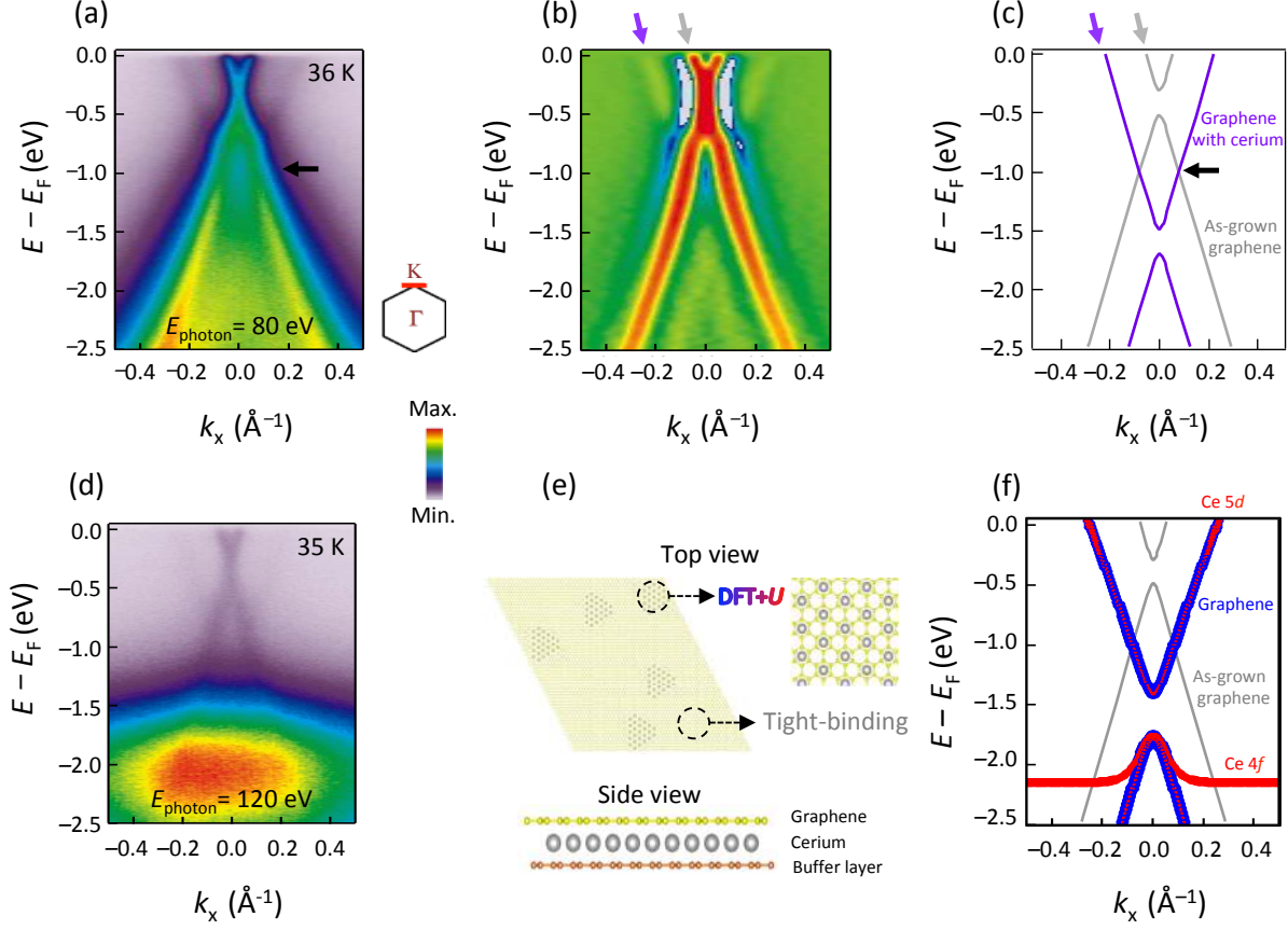
Figure 2: (a, b) An ARPES intensity map (a) and its second derivative (b) for Ce-intercalated graphene taken at 36 K using 80 eV photons across the K point perpendicular to the \Gamma K direction of the graphene unit cell denoted by the red line in the inset. (c) Tight-binding bands perpendicular to the \Gamma K direction with shifted Dirac energies corresponding to as-grown graphene (grey bands) and graphene with Ce (purple bands). (d) An ARPES intensity map for Ce-intercalated graphene taken at 35 K using 120 eV photons across the K point perpendicular to the \Gamma K direction. (e, f) A model structure for Ce-intercalated graphene (e) and a calculated band structure (f) perpendicular to the \Gamma K direction with U = 4 eV and J = 0.68 eV. The blue and red colors denote the electronic contribution from C and Ce orbitals, respectively. The grey bands are tight-binding bands for as-grown graphene.
