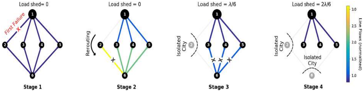
FIG. 2. Cascade in a six-node network with X_1 = 1 , X_j = 0 for j \geq 2 , \lambda > 3/4 . The four lower and upper line flows are \lambda/24 and 5\lambda/24 , respectively, with corresponding emergency limits 1/24 and 5/24 . The failure of an upper line causes the load on the adjacent lower line to surge to \lambda/6 > 1/24 , causing this line to trip (stage 2). This cutoff leads to the load on the three remaining lower lines to surge to \lambda/18 , causing them to trip as well (stage 3). After isolating nodes 2 and 6, the cascade ends with |A_1| = 4 and a total load shed of 2\lambda/6 (stage 4).
