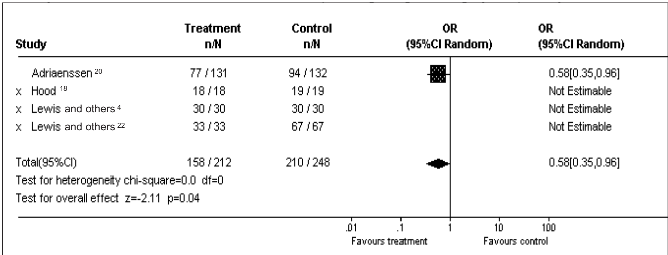
Figure 1: Results of the meta-analysis for the outcome absence of pain and infection at the end of the follow-up period (Forrest plot). n = number of patients showing outcome of interest, N = number of patients in treatment or control group, OR = odds ratio, CI = confidence interval, df = degrees of freedom.
