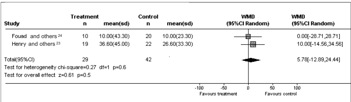
Figure 2: Results of the meta-analysis for the outcome mean pain at 3 days follow-up (Forrest plot). SD = standard deviation, WMD = weighted mean difference, CI = confidence interval, df = degrees of freedom.
