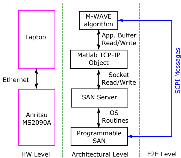
Fig. 3. Considered software-defined architecture for performing the EMF measurements.
