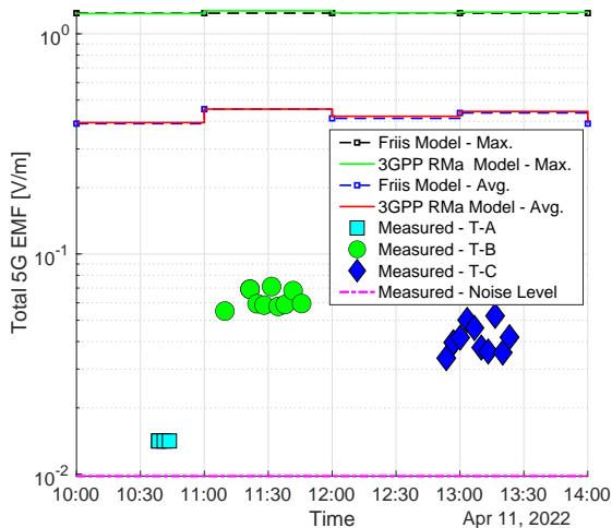
Fig. 10. Comparison among measured and simulated EMF levels.
