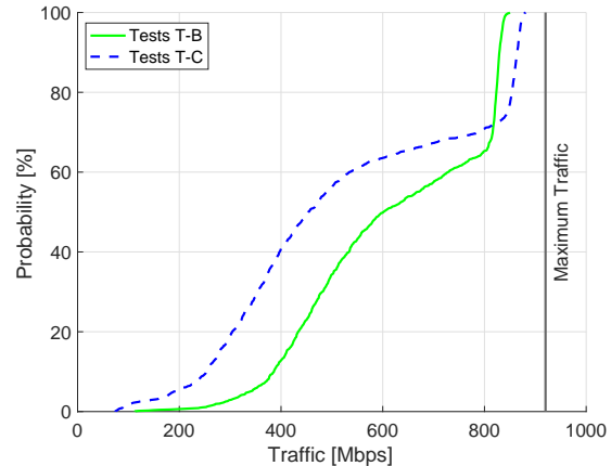
Fig. 11. ECDF of the instantaneous DL Throughput (T-B) and T-C tests).
