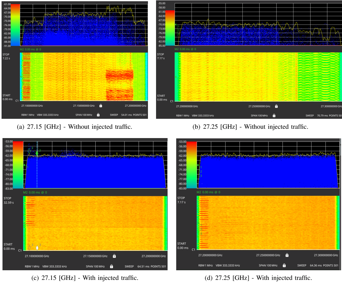
Fig. 6. Impact of traffic on the spectrum of the 5G mm-Wave carriers (subfigures best viewed in colors).
