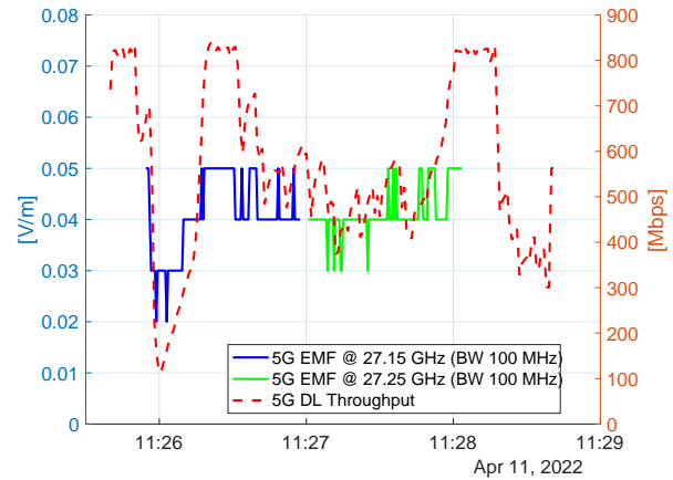
Fig. 8. DL Throughput and 5G mm-Wave EMF measurements vs. time for a given test.
