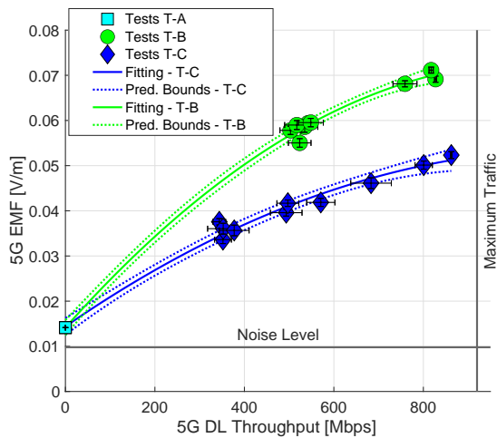
Fig. 9. mm-Wave 5G Exposure vs. DL throughput over the different tests.
