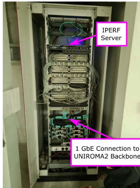
Fig. 2. Server installation at the Uniroma2 backbone.
