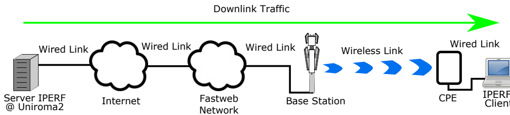
Fig. 1. End-hosts and network segments involved in the DL tests.
