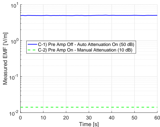
Fig. 14. 5G mm-Wave exposure with different SAN settings. The setting with pre-amplifier deactivated and 50 [dB] of attenuation (default level) leads to a large over-estimation of exposure levels.
