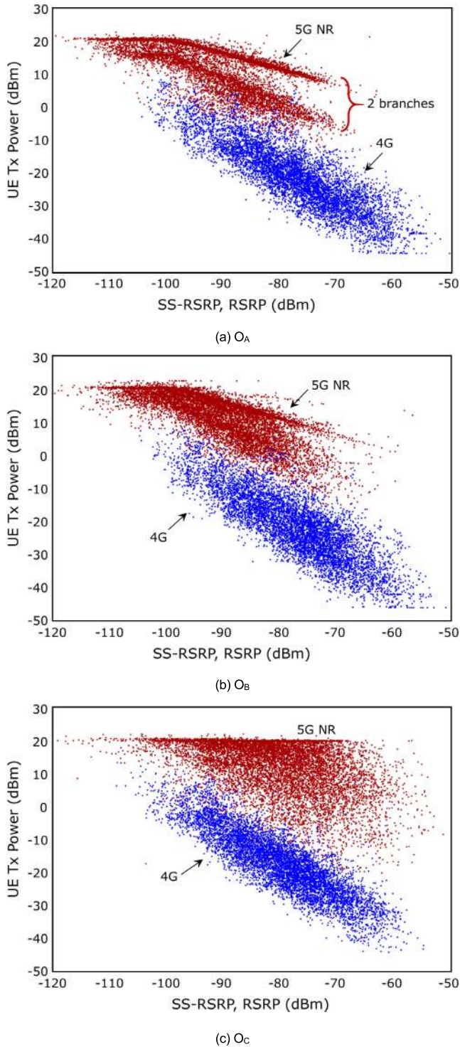
FIGURE 6. Scatter plot of UE-Tx power and SS-RSRP for 5G (RSRP for 4G). To reduce the plotting load caused by the large number of power samples ( 9 \times 10^5 to 1 \times 10^6 ), only 1% of the total number of samples were used in the plots.
