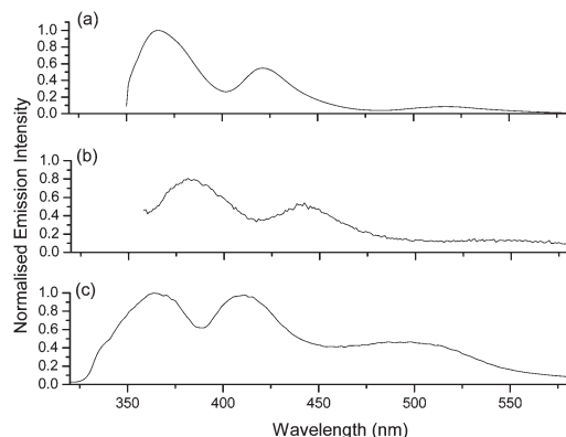
Fig. 3 (a) Emission spectrum of 1 in THF ( \lambda_{\text{exc}} = 303 nm); (b) emission spectrum of 2 in THF ( \lambda_{\text{exc}} = 325 nm); (c) emission spectrum of [\text{UCl}_4(\text{THF})_3] in THF ( \lambda_{\text{exc}} = 290 nm), all measured at 298 K (Raman bands have been subtracted).
