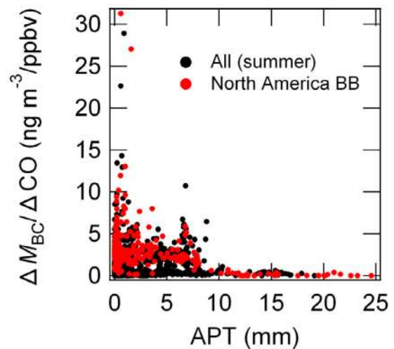
Figure 4. M_{BC}/\Delta \text{CO} ratios plotted versus APT during ARCTAS-B. The APT was calculated for 24 h prior to aircraft sampling.
