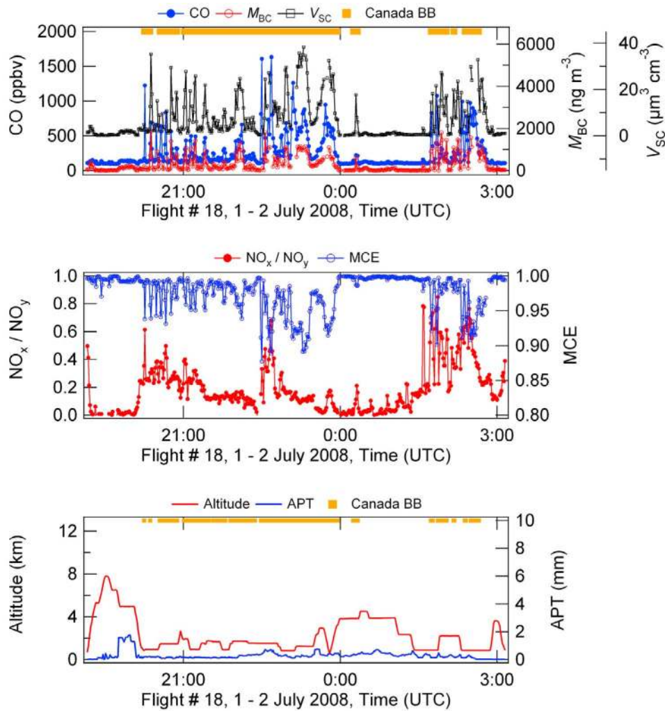
Figure 3. (top) Time series plots of CO, BC mass concentration ( M_{BC} ), volume concentration of LSP ( V_{SC} ), and identification of BB plumes. (middle) MCE and \text{NO}_x/\text{NO}_y ratio. (bottom) Precipitation (APT) and altitude of the DC-8 on 1–2 July.
