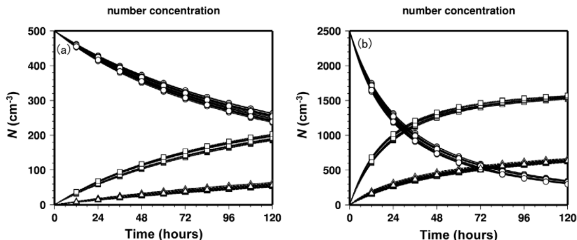
Figure 19. Total decay of N_{\text{LSP}} due to intramodal and intermodal coagulation, the decay due solely to intramodal coagulation ( \Delta N_{\text{LSP}} (intra)), and the decay due solely to intermodal coagulation ( \Delta N_{\text{LSP}} (inter)) for conditions of (a) N_{\text{LSP}} = 500 \text{ cm}^{-3} and (b) N_{\text{LSP}} = 2500 \text{ cm}^{-3} . \Delta N_{\text{LSP}} (intra) and \Delta N_{\text{LSP}} (inter) are shown as positive values. The other parameters for the initial lognormal size distribution (LNSD) are N_{\text{LSP}} = 500, 1500, \text{ and } 2500 \text{ cm}^{-3} ; N_{\text{BC}} = 0.1 \times N_{\text{LSP}} ; \text{CMD}_{\text{LSP}} = 200, 230, \text{ and } 250 \text{ nm} ; \text{CMD}_{\text{BC}} (\text{shell}) = 120, 160, \text{ and } 200 \text{ nm} ; \sigma_{\text{LSP}} = 1.2 \text{ and } 1.4 ; and \sigma_{\text{BC}} = 1.2 \text{ and } 1.3 .
