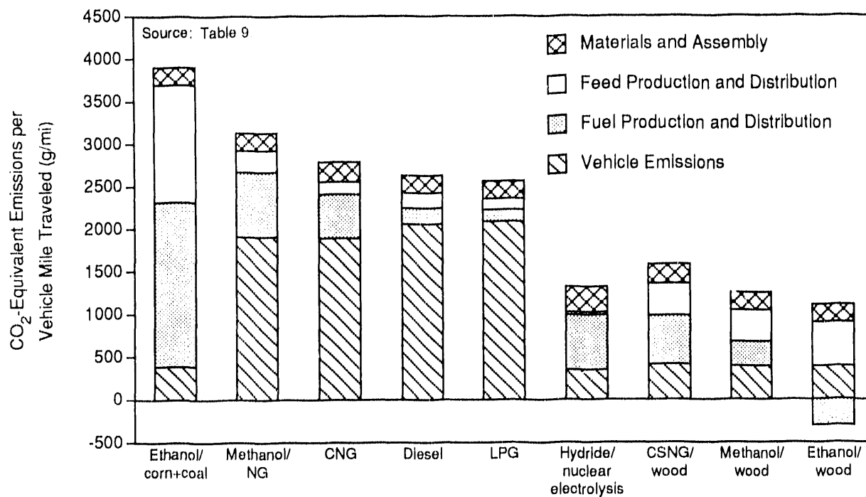
FIGURE 3 Total Fuel-Cycle, CO 2 -Equivalent Emissions for Heavy-Duty Vehicles
