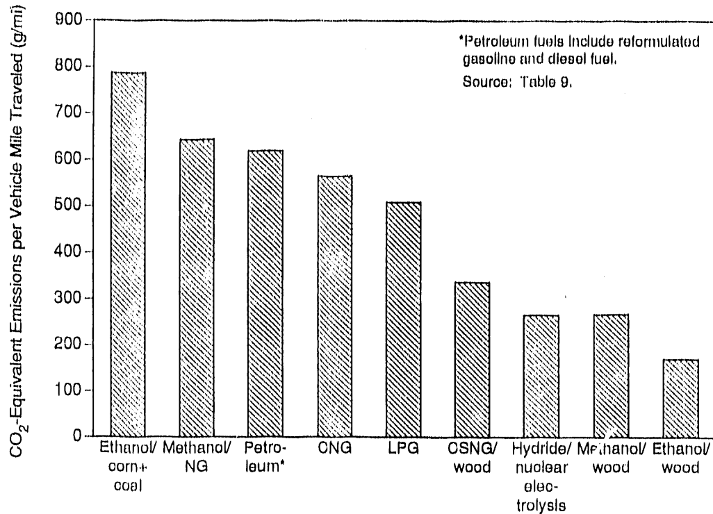
FIGURE 4 Total Fuel-Cycle, CO 2 -Equivalent Emissions for a Fleet of Light-Duty and Heavy-Duty Vehicles Combined
