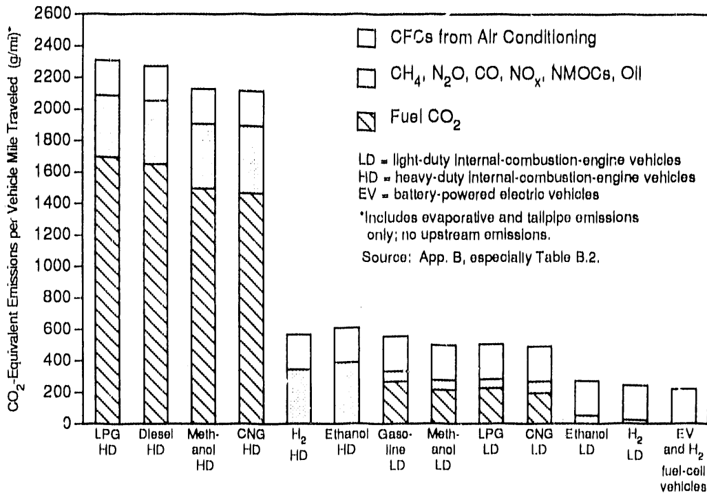
FIGURE 5 CO 2 -Equivalent Emissions from Vehicle End Use Only
