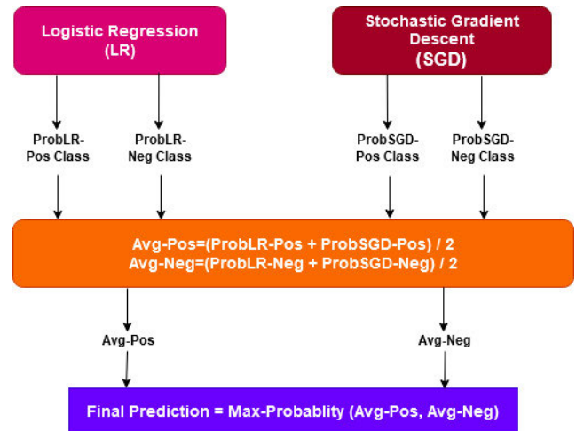
FIGURE 3. Proposed voting classifier architecture (LR-SGD).
