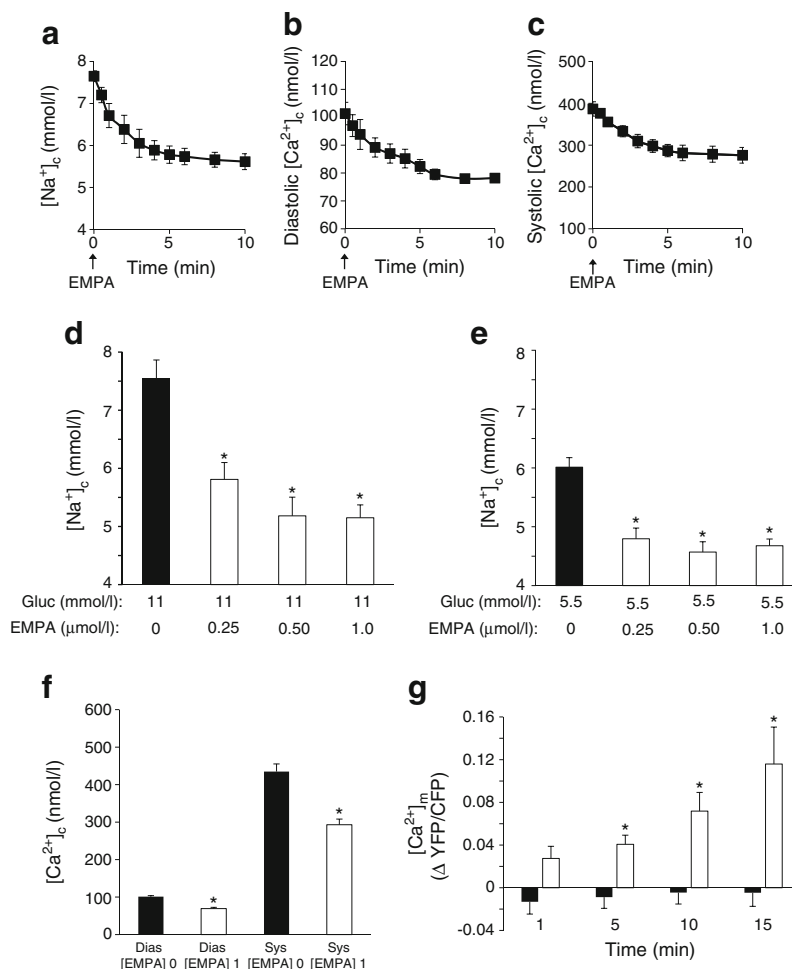
Fig. 1 EMPA effects on [Na^+]_c , [Ca^{2+}]_c and [Ca^{2+}]_m . ( a–c ) EMPA (1 \mu mol/l) acutely lowers ( a ) [Na^+]_c , and ( b ) diastolic [Ca^{2+}]_c and ( c ) systolic [Ca^{2+}]_c in rabbit cardiomyocytes. ( d,e ) Effects of EMPA (3 h incubation) on [Na^+]_c at ( d ) 11 mmol/l and ( e ) 5.5 mmol/l glucose (Gluc), respectively. * p < 0.05 vs 0 \mu mol/l EMPA, ANOVA with Dunnett's post hoc tests. ( f ) Effects of EMPA (3 h pre-incubation; [EMPA] 1) on diastolic (Dias) and systolic (Sys) [Ca^{2+}]_c at 11 mmol/l glucose. * p < 0.05 vs 0 \mu mol/l EMPA ([EMPA] 0), unpaired t test. ( g )
