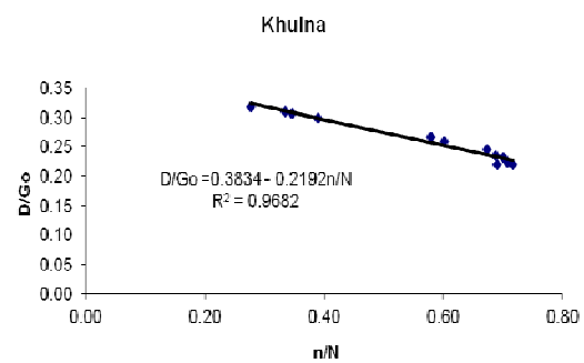
Figure 6. Correlation between n/N and D/Go for coefficient c' and d'
