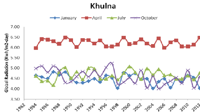
Figure 2. Year to year seasonal variation of Global solar radiation for Khulna
