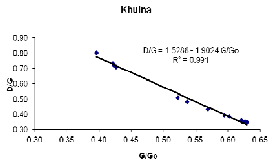
Figure 5. Correlation between G/Go and D/G for coefficient c and d
