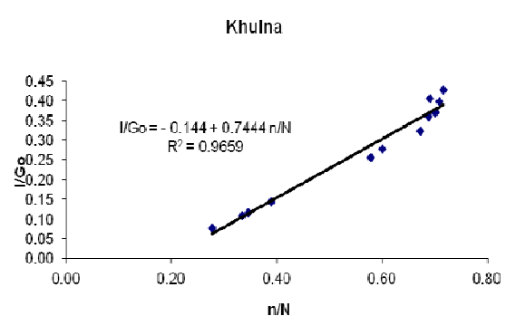
Figure 8. Correlation between n/N and I/Go for coefficient e' and f'
