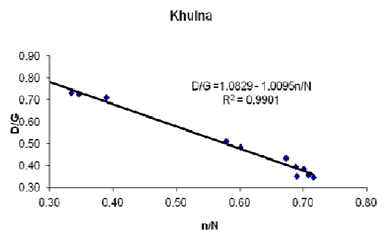
Figure 9. Correlation between n/N and D/G for coefficient co and do
