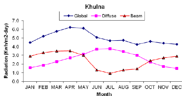
Figure 1. Monthly variation of Global, diffuse and beam solar radiation on a horizontal surface for Khulna
