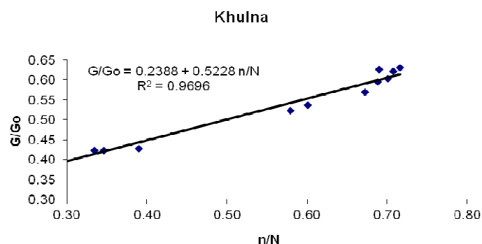
Figure 4. Correlation between n/N and G/Go for coefficient a and b
