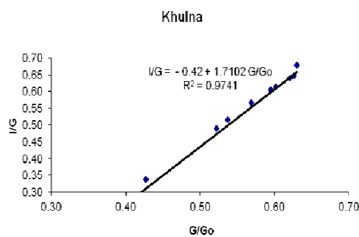
Figure 7. Correlation between G/Go and I/G for coefficient e and f
