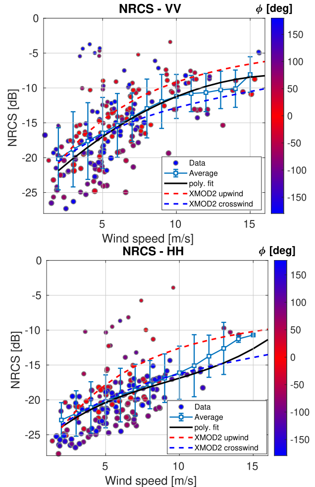
Fig. 10. NRCS dependence on ERA5 wind speed for VV (top) and HH (bottom) polarization. Solid lines are the polynomial fit (black) and average (blue) with error bars ( \pm\sigma_{U_D} ). Dashed line is XMOD2 simulated with mean incidence angle (33.7° for VV and 40° for HH). The size of data points increases with incidence angle from 20° to 50° and the color indicates the relative wind direction (see colorbar).
