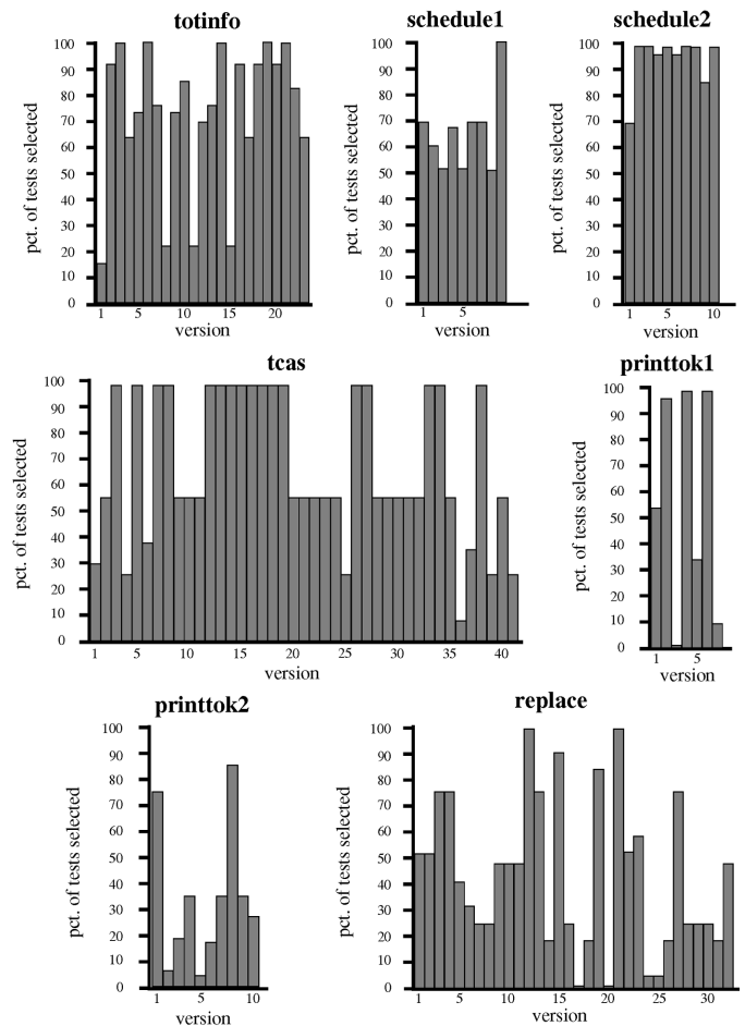
Fig. 2. Test selection statistics for Study 1.
