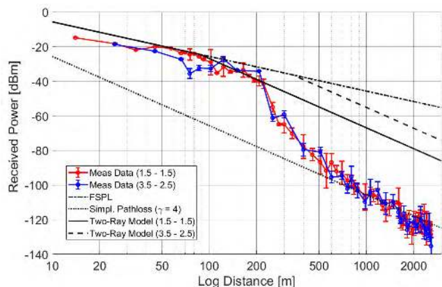
FIGURE 8. Received power for both measurement datasets plotted with the simplified path-loss model (5) as well as the Two-Ray model (3) for comparison.
