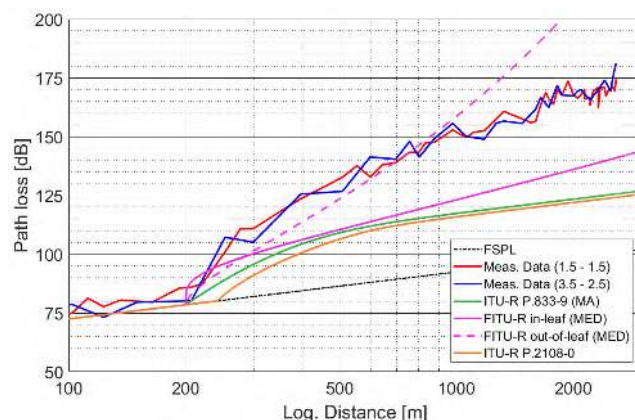
FIGURE 10. Comparison between foliage excess loss models added with FSPL and measurement data.
