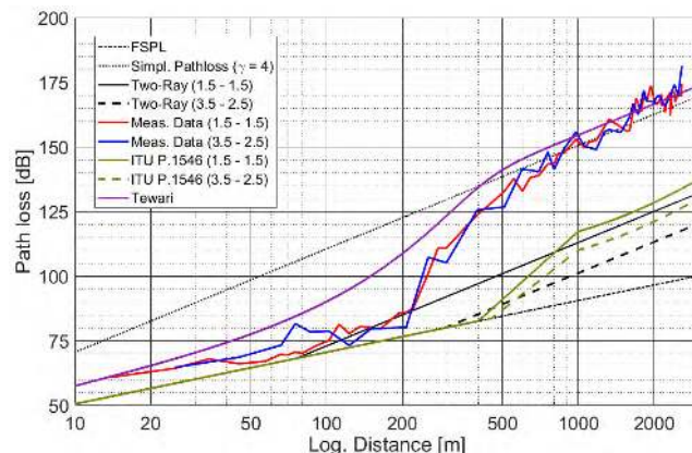
FIGURE 9. Comparison between terrain path-loss models and measurement data.
