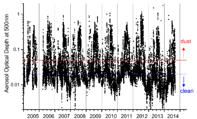
Figure B3. Time series of the AERONET aerosol optical depth at 500 nm reported for Izaña (2005–2012: level 2.0; 2013 and 2014: level 1.5).
