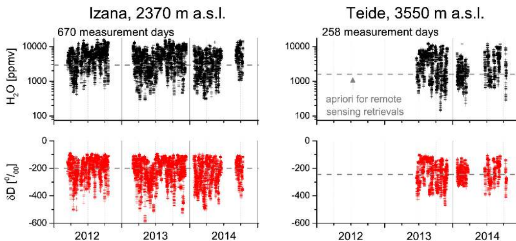
Figure 2. H_2O (upper panel) and \delta D data (bottom panel) as measured by the Picarro instruments on Tenerife between midnight and 1 hour after sunrise. The depicted data are 10 min averages obtained during a large amount of different days (numbers as given in the panel). For comparison we also depict the a priori values used for the MUSICA NDACC/FTIR and METOP/IASI remote sensing retrievals (grey dashed lines).
