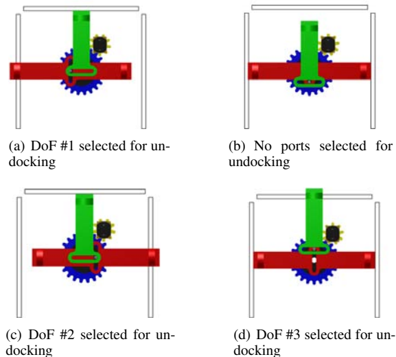
Fig. 5. Docking Key Connector Selection
