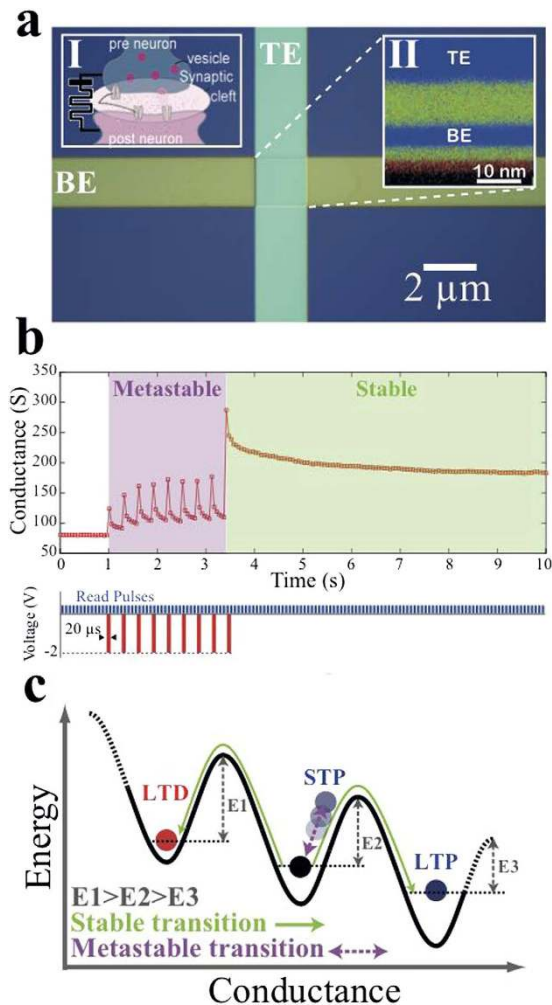
Figure 1. Solid-state TiO 2 ReRAM memristors can support volatile switching, enabling the emulation of short-term plasticity. A top-view of a 2 \times 2 \mu\text{m}^2 active area and 10 nm thick TiO 2 cross-bar architecture is shown in (a), with insets I and II respectively depicting cross-sections of a chemical synapse and a pristine memristor (blue denotes the Pt TE and BE that correspond to pre- and post-synaptic terminals, with green and red corresponding to Ti and O 2 species that can be displaced within the functional core). Schematic illustrations of possible conduction mechanisms that can induce a non-volatile increase (decrease) in the device's conductance, corresponding to an LTP (LTD) response, as depicted in and (b) metastable transitions precede both cases, with potentiation (STP) captured respectively. A transition from volatile to non-volatile programming, as described in (b), is shown in (c) where identical voltage pulses initially trigger volatile switching and eventually a non-volatile state transition.
