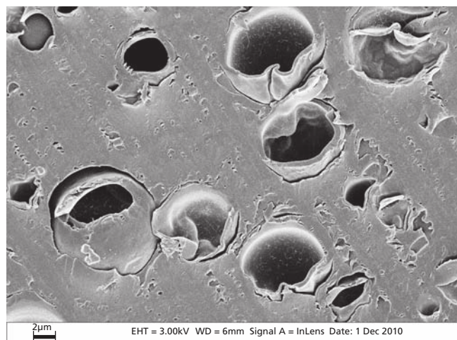
Figure 10. Cross-section biocide-filled core/shell containers with the PU shells in the dried polyepoxy coating matrix. Liquid core contained 10 wt% solution of 4'-5-dichloro-2-n-octyl-4-isothiazolin-3-one (DCOIT) in aromatic hydrocarbons.
