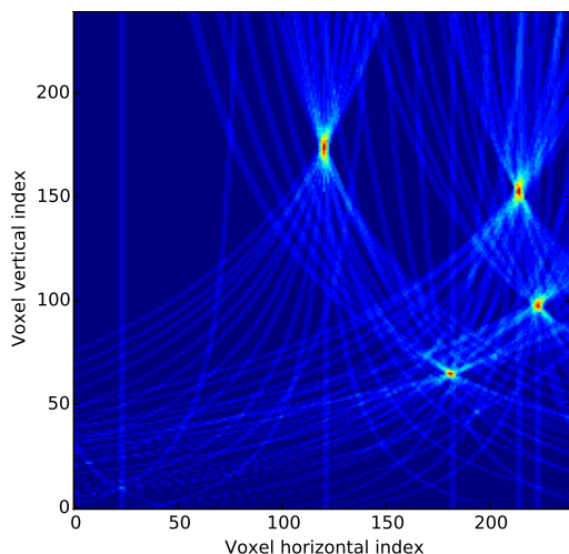
(c) Ray density using projective voxel grid, equispaced in depth (voxel vertical index). The width of each ray is constant along the depth.
