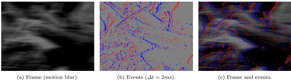
Fig. 12: High-speed experiment . Frame and the events from the DAVIS at 376 pixels/s. The frame suffers from motion blur, while the events do not, thus preserving the visual content.
