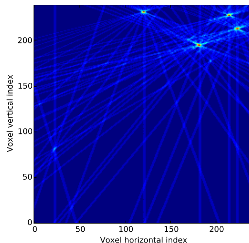
(d) Ray density using projective voxel grid, equispaced in inverse depth (voxel vertical index). As in Fig. 8c, the width of each ray is constant along the depth.
