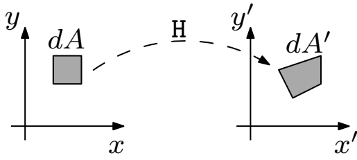
Fig. 18: Result 1. A homography \mathbf{H} maps points to points and lines to lines. Area elements are transformed according to dA' = |\mathbf{J}|dA , where \mathbf{J} is the Jacobian of the homography \mathbf{H} .
