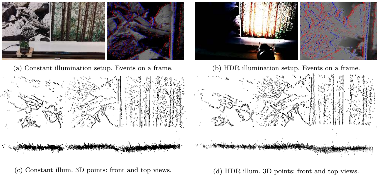
Fig. 11: HDR experiment : Top: Scene and illumination setups, with the DAVIS on the motorized linear slider (a) and a lamp (b). Sample frames show under- and over-exposed levels in HDR illumination (b). By contrast, the events (overlaid on the frames) are unaffected, due to the high dynamic range of the event sensor. Bottom: reconstructed point clouds.
