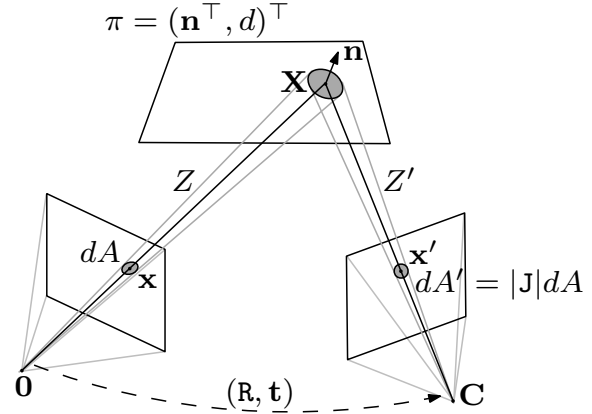
Fig. 19: Result 2. Relation of area elements induced by a planar homography: dA' = |\mathbf{J}|dA , where \mathbf{J} is the Jacobian of the planar homography, and Z, Z' are the depths of the scene point \mathbf{X} with respect to the two cameras, respectively.
