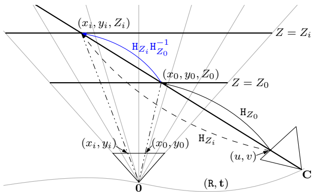
Fig. 9: Efficient event back-projection in Algorithm 1. An event with coordinates (u, v) is mapped onto the depth plane Z = Z_i of the projective DSI in two steps: first, it is mapped to the depth plane Z = Z_0 via \mathbf{H}_{Z_0} and then it is mapped to Z = Z_i via the similarity \mathbf{H}_{Z_i} \mathbf{H}_{Z_0}^{-1} in (15). In the figure, the notation x_i = x(Z_i) and y_i = y(Z_i) is used for brevity.
