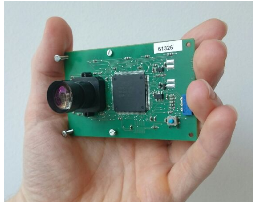
Fig. 1: The event camera “eDVS” produced by iniLabs.
