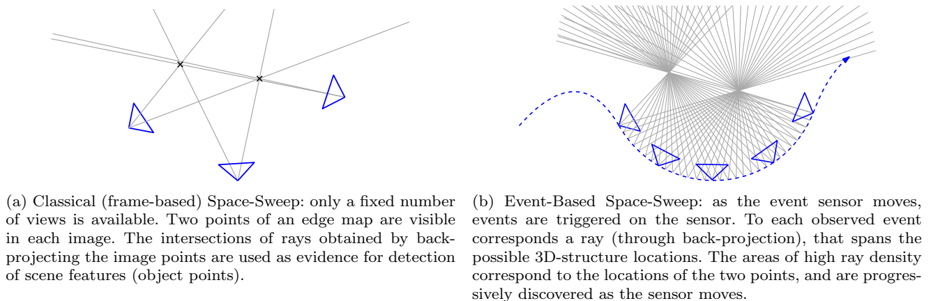
Fig. 3: Comparison of the back-projection step in classical Space-Sweep and Event-Based Space-Sweep. This is a 2D illustration with the scene consisting of two points.
