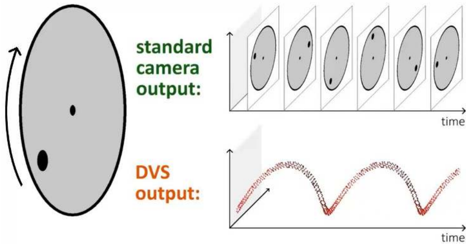
Fig. 2: Comparison of the output of a standard camera and an event camera (DVS) when viewing a spinning disk with a black circle. The standard camera outputs frames at a fixed rate, thus sending redundant information when no motion is present in the scene. In contrast, event cameras are data-driven sensors that output pixel-level brightness changes with microsecond latency. Therefore, they do not suffer from motion blur and produce no output if there is no visual change in the scene. An animated version can be found here: https://youtu.be/LauQ6LWTkxM .
