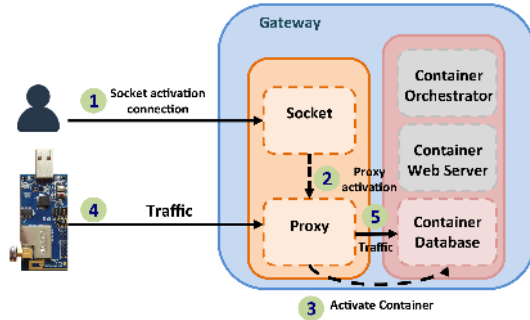
Fig. 3: Container activation through socket/proxy connection.
