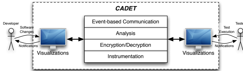
Figure 1. High-level view of the five areas of research for our approach.
