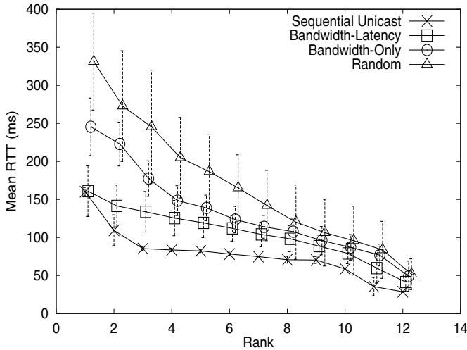
Figure 7: Mean RTT versus rank at 1.2 Mbps source rate for the Primary Set of machines
