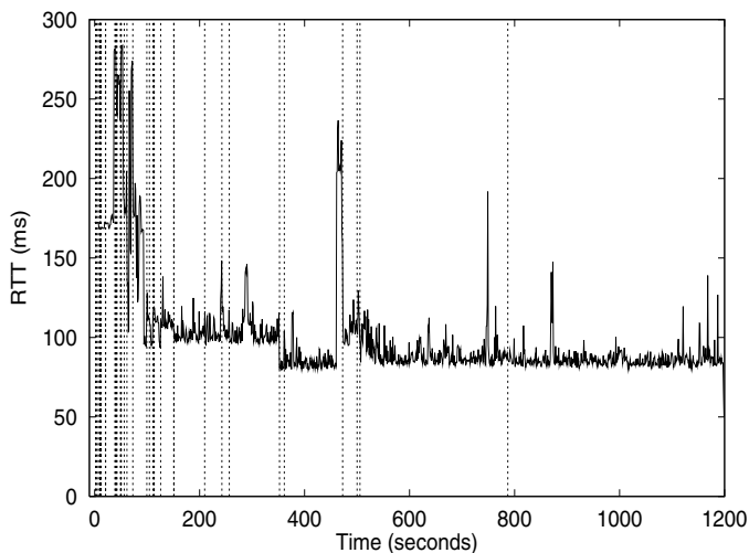
Figure 4: Mean RTT averaged over all receivers as a function of time.
