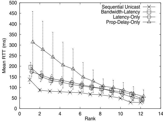
Figure 9: Mean RTT versus rank at 2.4 Mbps source rate for the Primary Set
