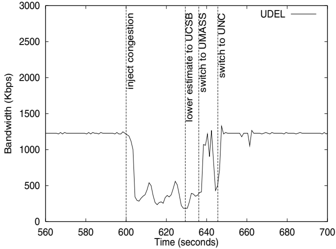
Figure 12: An example demonstrating adaptation to network congestion in one controlled experiment.
