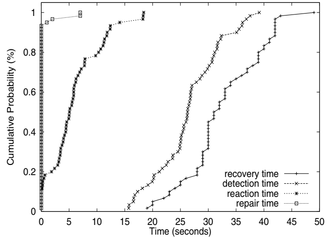
Figure 13: Cumulative distribution of recovery time and its components for the victim hosts
