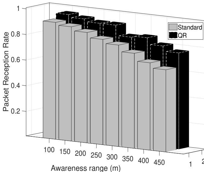
Fig. 4. Reception rate of dual interface vehicle according to the awareness range of proposed QR and standard relaying protocol
