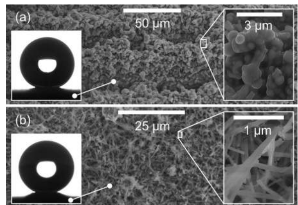
FIG. 1. Scanning electron microscope (SEM) images of (a) the laser-etched microstructured copper surface (300 \times ; top-right inset at 4000 \times ) and (b) the chemically etched nanostructured copper surface (800 \times ; top-right inset at 15000 \times ). Insets at bottom left of each frame show a static 5 \mu l droplet resting on the respective surface in the Cassie-Baxter state.
