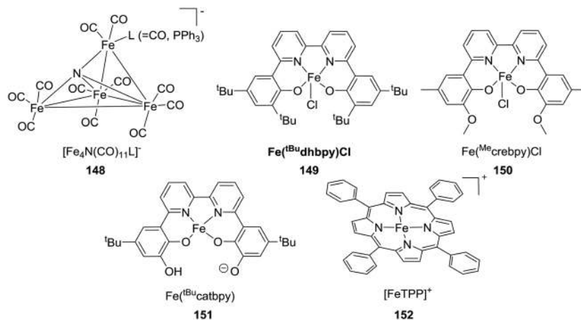
Fig. 45 Fe-based molecular electrocatalysts for selective reduction of \text{CO}_2 to formate.
