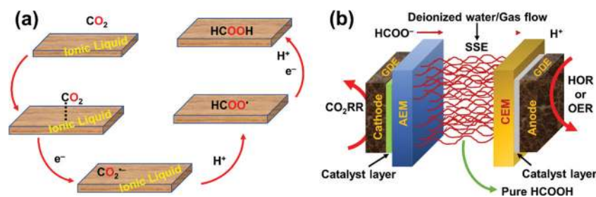
Fig. 34 (a) Possible reaction mechanism for the e\text{CO}_2\text{RR} towards FA formation in IL containing catholytes on the electrode surface. 184 (b) Schematic illustration of an all solid-state reactor containing solid electrolyte for the e\text{CO}_2\text{RR} to pure FA. 185,186
