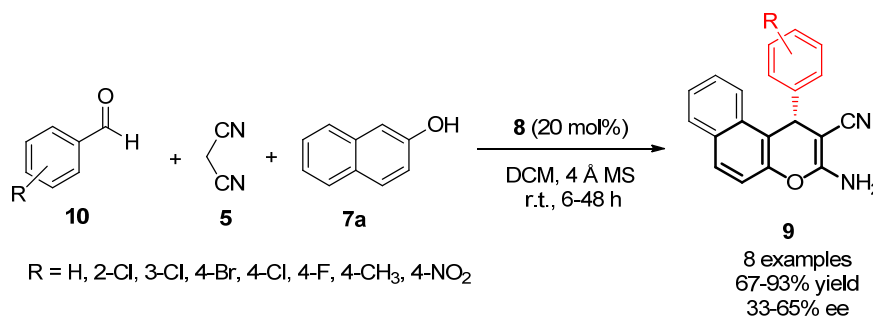
Scheme 3. Multicomponent enantioselective synthesis of benzochromene derivatives 9 .
