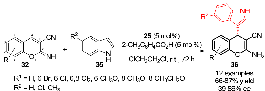
Scheme 17. Enantioselective synthesis of 4-(indol-3-yl) derivatives 36 .
