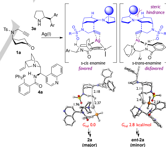
Scheme 5. Computed (SMD-M06-2X/def2-TZVP//def2-SVP) transition structures for C-C formation of major and minor enantiomers.
