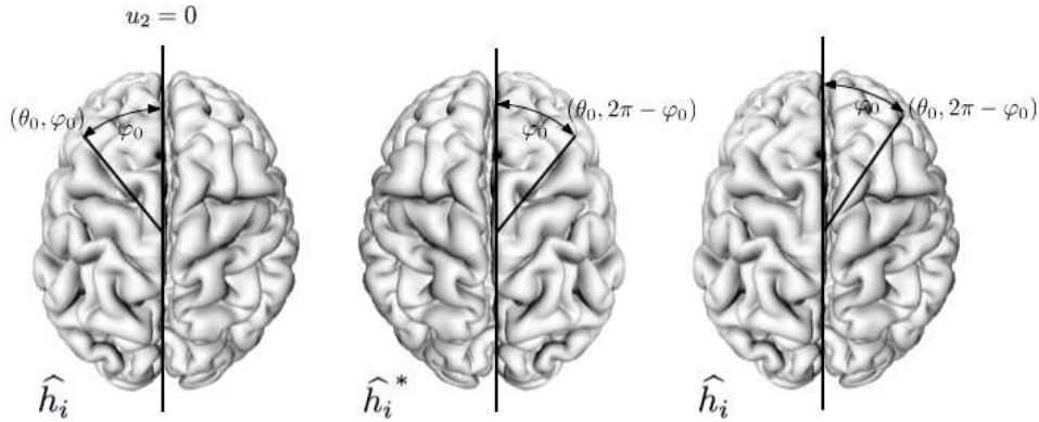
Figure 4. The point \widehat{h}_i(\theta_0, \varphi_0) (left) corresponds to \widehat{h}_i^*(\theta, 2\pi - \varphi_0) (middle) after mirror reflection with respect to the midsagittal cross section u_2 = 0 . From the spherical harmonic correspondence, \widehat{h}_i^*(\theta, 2\pi - \varphi_0) corresponds to \widehat{h}_i(\theta, 2\pi - \varphi_0) (right). This establishes the mapping from the left hemisphere to the right hemisphere in least squares fashion.
