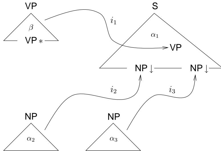
Figure 2.2 A Derivation Step
