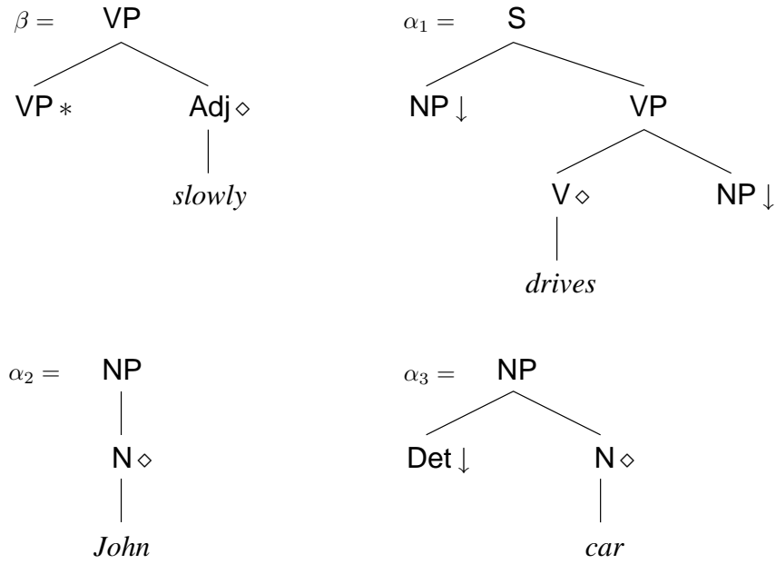
Figure 2.1 An Example Grammar
