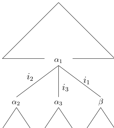
Figure 2.3 A Derivation Tree
