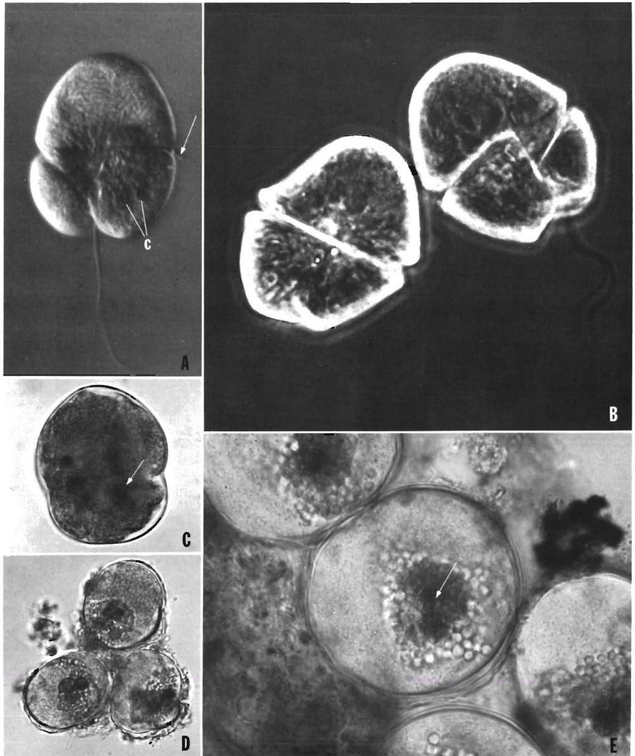
Fig. 9. Gyrodinium uncatenum . Major life cycle stages in individuals isolated from the Potomac River of Chesapeake Bay. (A) Nomarski interference micrograph ( \times 1064 ) of a typical vegetative cell characterized by numerous, closely spaced chloroplasts (c), and 2 flagella (1 transverse [arrow], 1 posterior). (B) Two planozygotes characterized by 2 distinct posterior flagella in addition to 2 transverse flagella (not visible). Red pigmentation granules have developed in the hypocone (phase contrast, \times 1028 ). (C) Late planozygote/early hypnozygote characterized by rounding of the cell, red pigmentation granules (arrow), and a decrease in motility ( \times 800 ). (D) Hypnozygote cluster showing outer membrane separated from inner smooth cell wall ( \times 518 ). (E) Hypnozygotes at higher magnification with interior of cell containing red pigmentation granules (arrow), and surrounded by numerous oil droplets ( \times 1332 )
