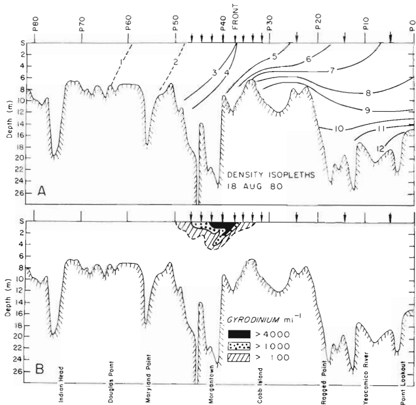
Fig. 6. Longitudinal section through spine of Potomac estuary; August, 1980. (A) Density isopleths represented as solid lines with frontal region (foamline) evident near P35. (B) Gyrodinium uncatenum . Individuals \text{ml}^{-1} showing association with frontal region
