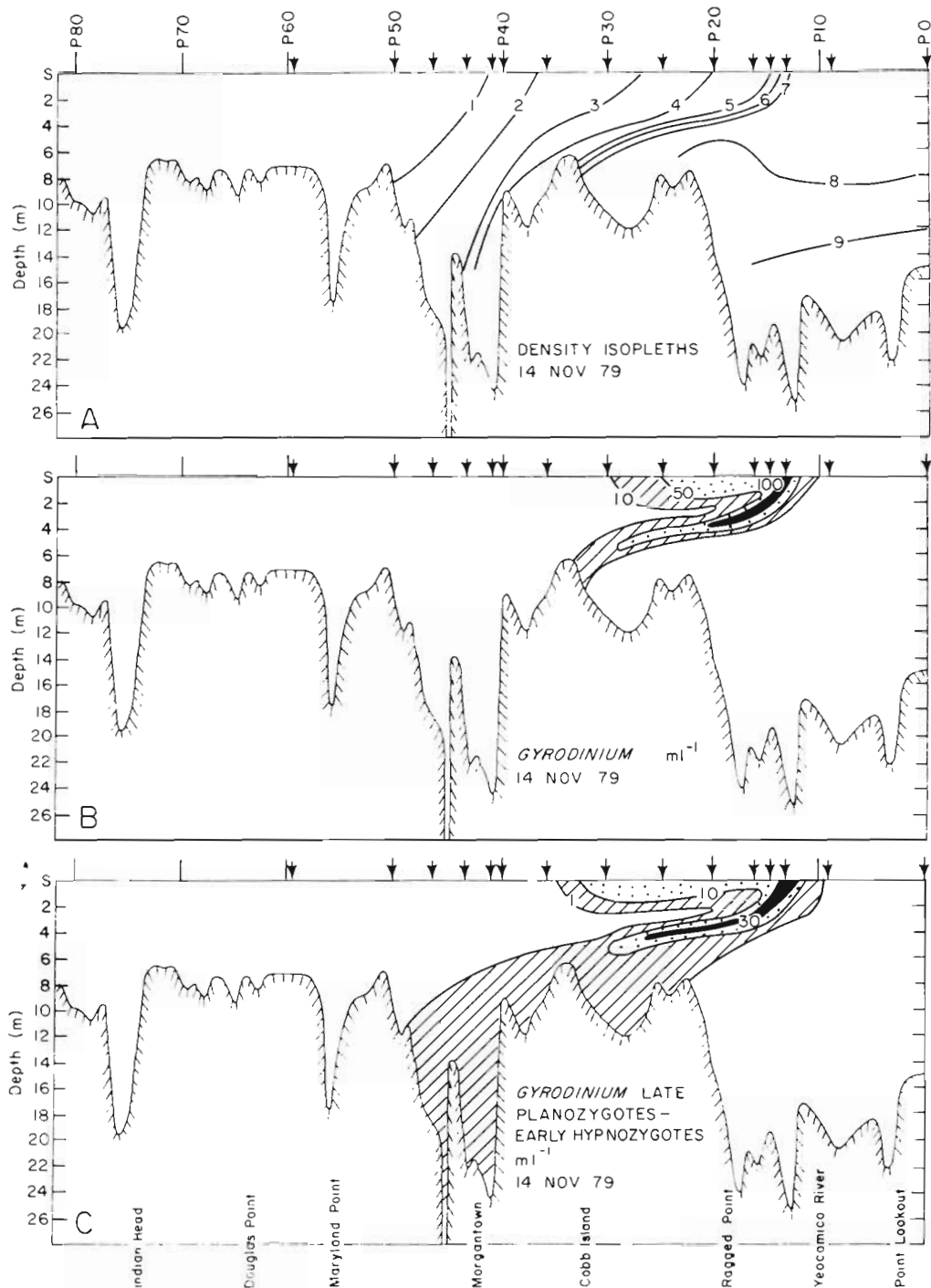
Fig. 11. Longitudinal cross-section through spine of Potomac River; 14 November, 1979. Arrows: vertical profile station locations. (A) Density isopleths indicating upstream penetration of higher-salinity bay water to Station P50. A surface frontal region exists in the region of P15 as indicated by the 5, 6 and 7 \sigma_t isopycnals breaking the surface. (B) Gyrodinium uncatenum . Optical counts of motile individuals, including planozygotes and vegetative cells. (C) Ditto. Optical counts of late planozygotes/early hypnozygotes
