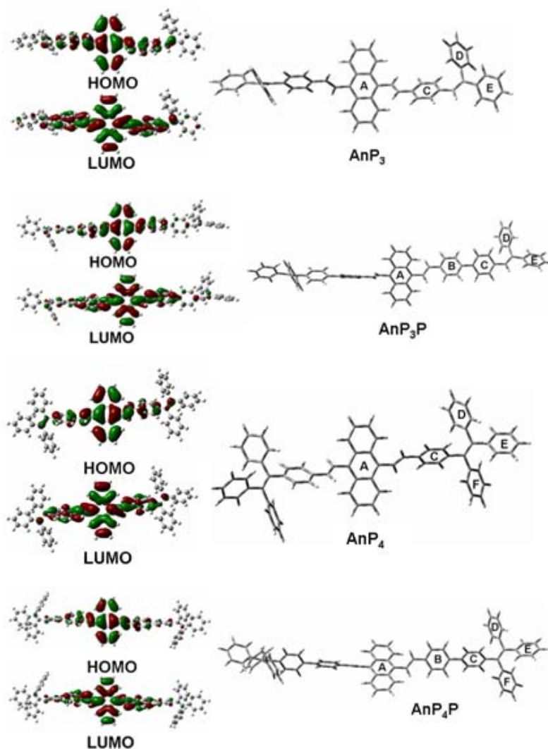
Fig. S1 Calculated spatial electron distributions of LUMOs and HOMOs (left); and the optimized structure of the compounds (right).
