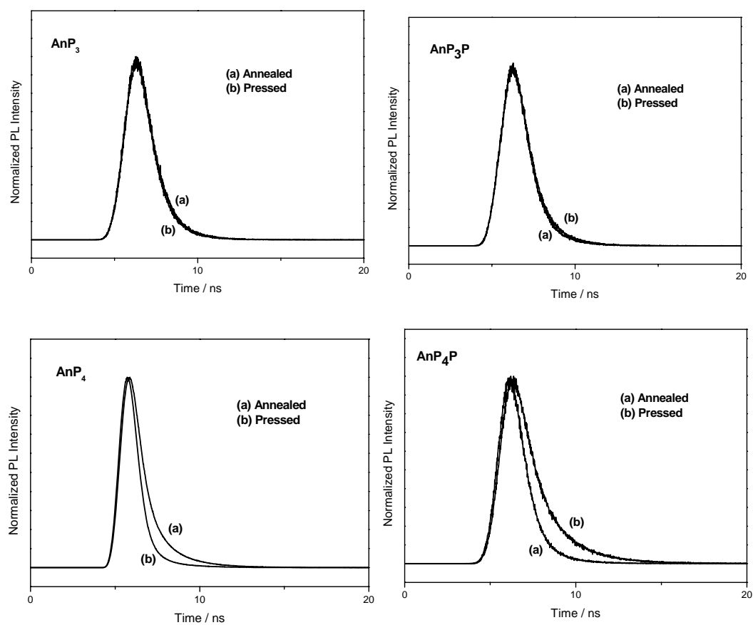
Fig. S2 Time-resolved emission decay curves of the annealed and pressed of AnP 3 , AnP 3 P, AnP 4 and AnP 4 P samples.
