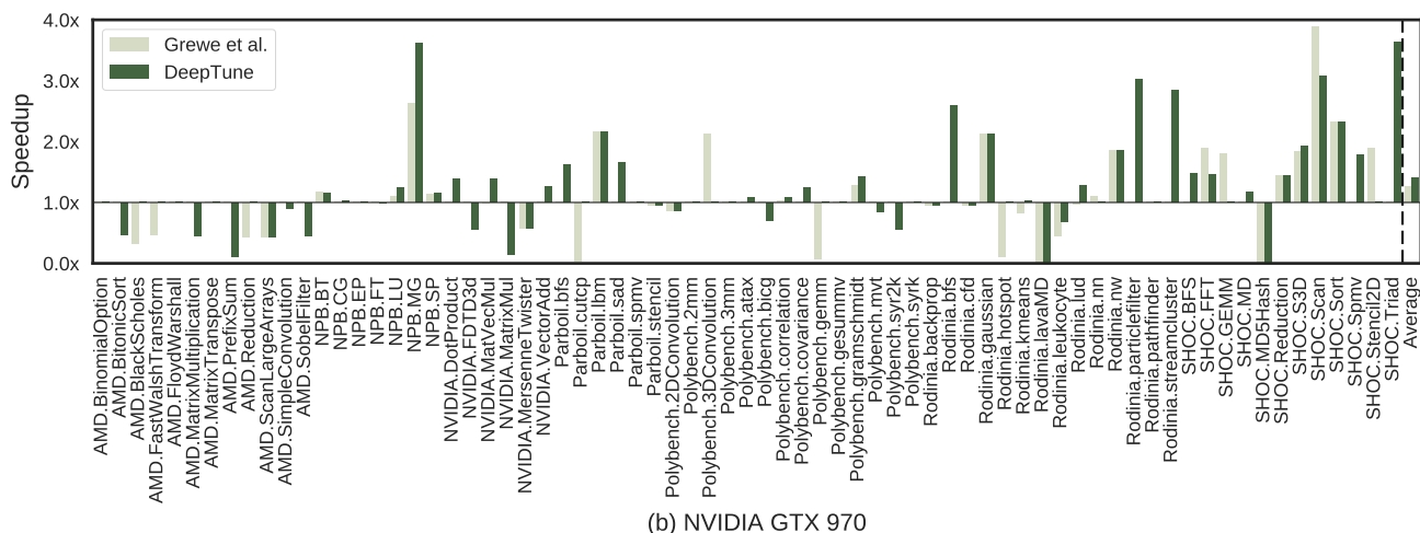
Figure 7: Speedup of predicted heterogeneous mappings over the best static mapping for both platforms. In (a) DeepTune achieves an average speedup of 3.43x over static mapping and 18% over Grewe et al. In (b) the speedup is 1.42x and 13% respectively.
