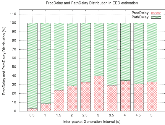
Fig. 10. ProcDelay and PathDelay Distribution – IGI from 0.5 to 5s
