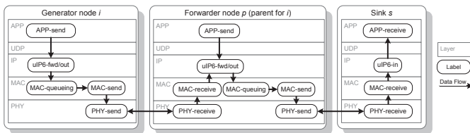
Fig. 2. EED estimation – WSN nodes' interaction
