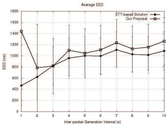
Fig. 14. Average EED
