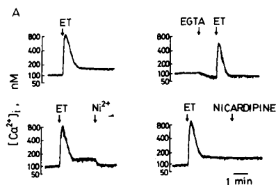
Figure 2. Effect of ET on [Ca^{2+}]_i . A , Effects of EGTA ( 2 \times 10^{-3} M), Ni^{2+} ( 1 \times 10^{-3} M), and nicardipine ( 1 \times 10^{-6} M) on 10^{-7} M ET-induced increase in [Ca^{2+}]_i . Test substances were applied at arrows and were present throughout each recording. Tracings are representative of at least four experiments. B , Dose-response curve of ET-induced increases in [Ca^{2+}]_i . Each value expresses the mean of four to six determinations.
