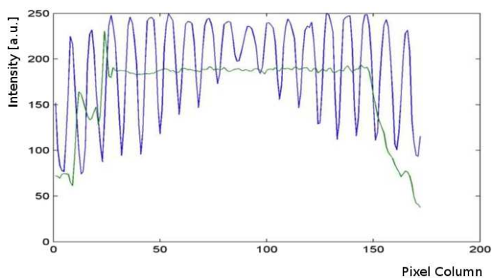
Figure 6. light distribution of an X-ray excited LYSO crystal measured with a CCD camera with (blue) and without (green) optical elements.
