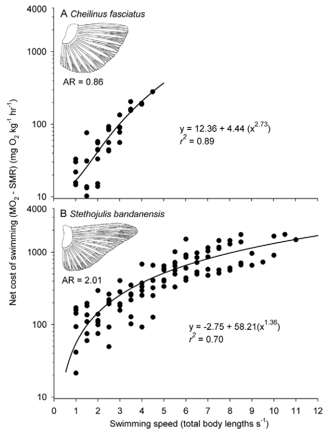
Figure 2. Net cost of swimming for two species of reef fish with alternate pectoral fin shapes , as indicated by the aspect ratio (AR), displayed different increases in oxygen consumption with speed as indicated by the semi-log plots for (A) Cheilinus fasciatus and (B) Stethojulis bandanensis fitted with the hydrodynamics-based power equation ( MO_2 - SMR = a + b U^c ) [3]. A low exponent value (c) for S. bandanensis indicates a very high efficiency of locomotion with increasing speed compared to other bony fishes (Table 1). doi:10.1371/journal.pone.0054033.g002
