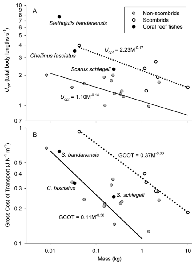
Figure 3. Comparative energetic swimming performance of bony fishes. Three coral reef and sixteen other non-scombrid fishes are presented alongside six scombrid (tuna-like) fishes of varying body mass on log-log plots of (A) Optimum swimming speed ( U_{opt} ) and (B) Gross cost of transport (GCOT) incurred by each species at their optimum swimming speed ( U_{opt} ). Dotted and solid lines denote mass- U_{opt} and mass-GCOT power functions [after 3, 6] for scombrid and non-scombrid fishes, respectively (note the range of temperatures encompassed within the underlying data in Table S1 [5,8,22–24,26–32], which reflect the conditions experienced by each species performing in the wild). Note S. bandanensis is well above the scombrid U_{opt} trend (A, dotted line), but has the same (much lower) GCOT as similar-sized non-scombrid fishes swimming four times slower (B, solid line). doi:10.1371/journal.pone.0054033.g003
