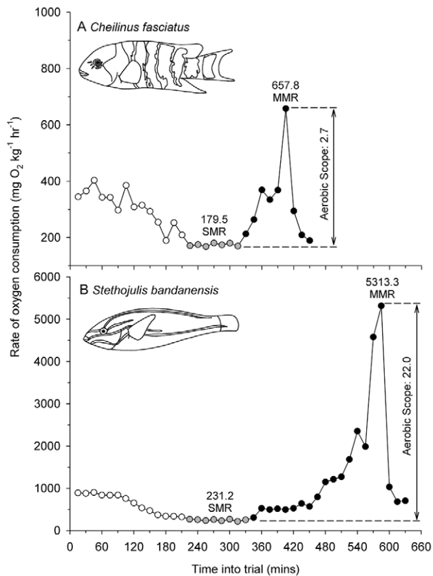
Figure 1. Rate of oxygen consumption against time in a swimming speed trial for (A) Redbreasted wrasse Cheilinus fasciatus (11.5 cm total body length) and (B) Bluelined wrasse Stethojulis bandanensis (10.5 cm). Factorial aerobic scopes are provided, which is the difference between maximum metabolic rate (MMR) during the trial (highest black dot) and the standard metabolic rate (SMR, grey dots), divided by SMR. Note the different y-axis scales, and rapid MO_2 drop on trial completion (last three dots) indicating minimal excessive post-exercise oxygen consumption (EPOC). doi:10.1371/journal.pone.0054033.g001
