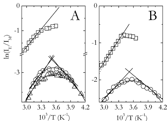
Figure 5. Arrhenius plots for the ratio I_E/I_M obtained in ethanol (O), acidified ethanol ( \Delta ), and water ( \square ) for (A) compound L1 and (B) compound L2 . The parabolic lines accompanying the experimental data are just meant to be guidelines for the eye.
