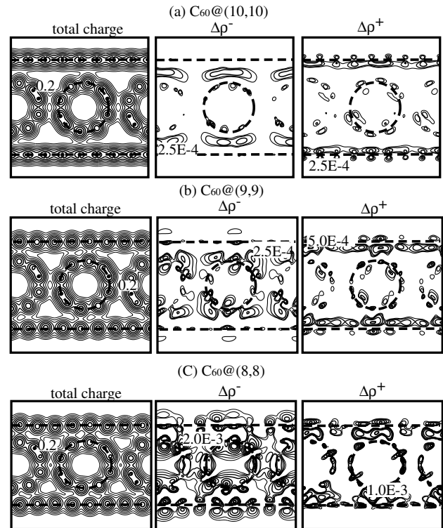
FIG. 4. Contour plots of the total valence charge density of C_{60}@ (n, n) . (a) n = 10 , (b) n = 9 , and (c) n = 8 . The contour plot of more negatively charged (electron rich) area, \Delta\rho^- , and that of the more positively charged, \Delta\rho^+ , than a simple sum of two self-consistent charge densities of the tubes and C_{60} are also shown. Each contour represents twice (or half) the density of the adjacent contour lines. The values shown in figures are in units of e/(\text{a.u.})^3 .
